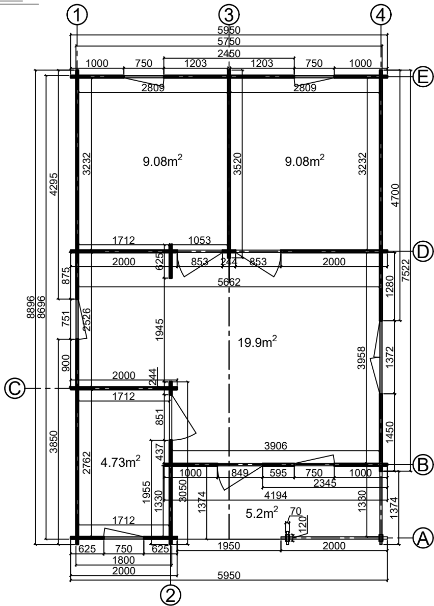
Floor plan
