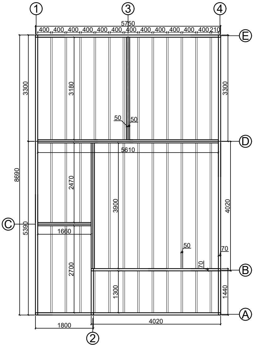
Base plan
