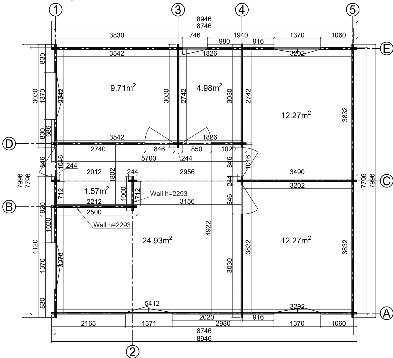
Floor plan
