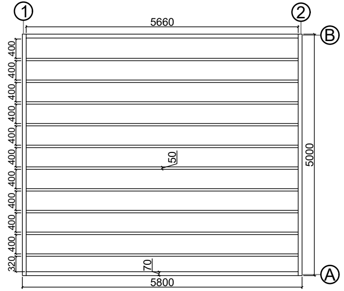
Base plan
