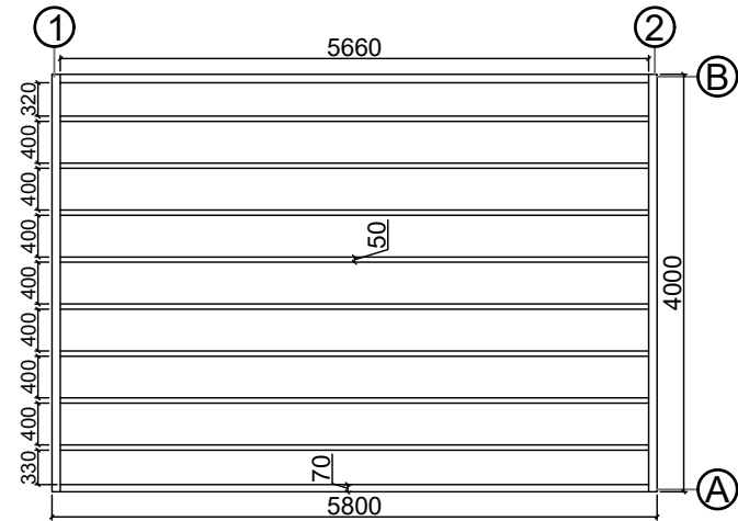
Base plan
