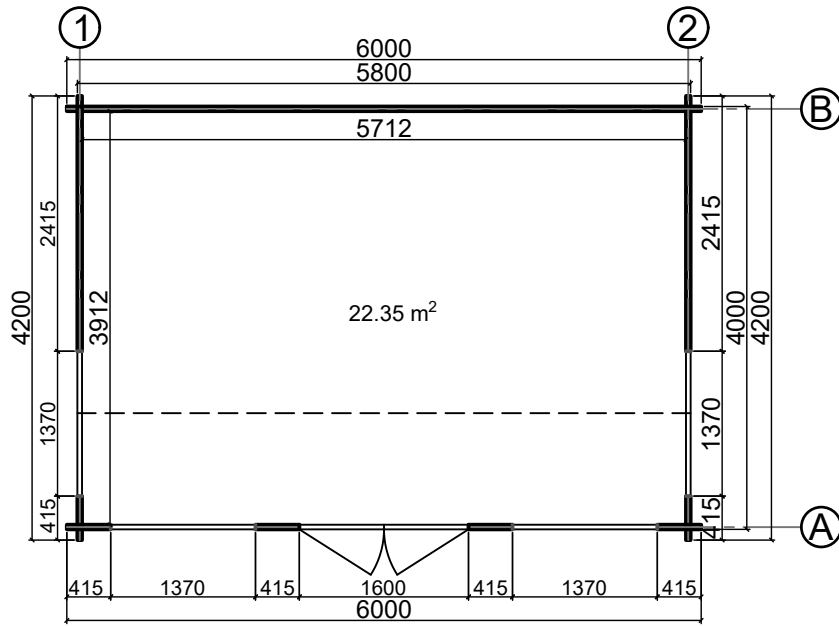
Floor plan
