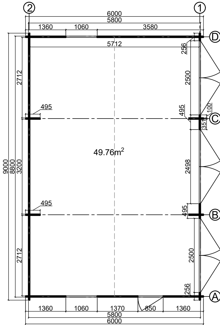
Floor plan
