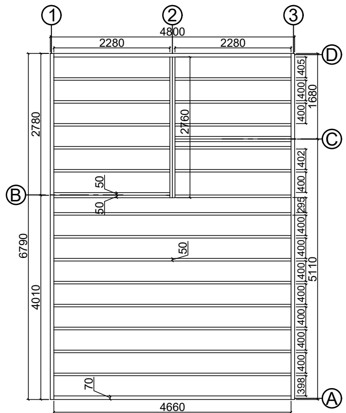
Base plan
