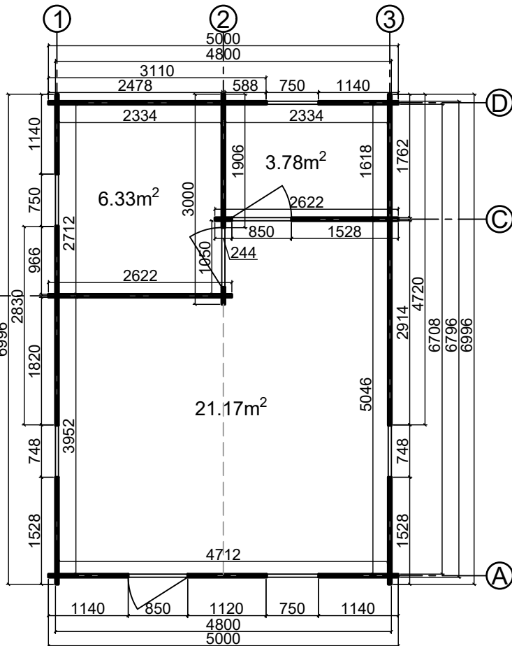
Floor plan
