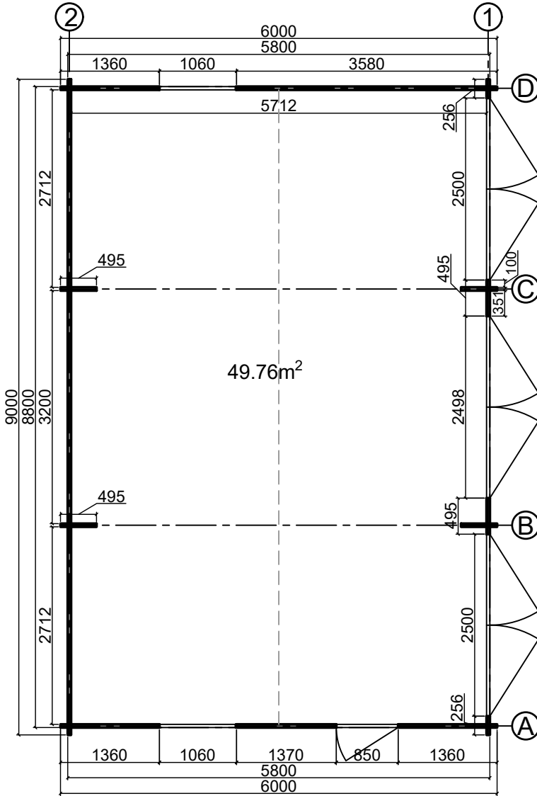
Floor plan
