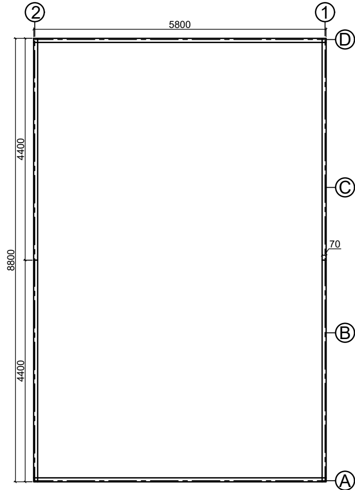
Base plan
