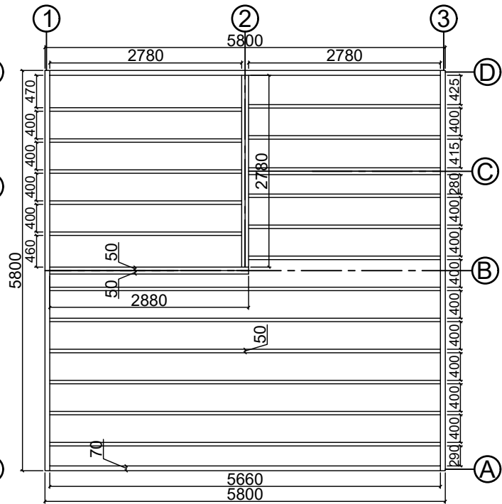
Base plan
