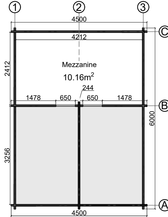
Mezzanine plan
