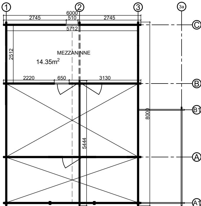
Mezzanine plan
