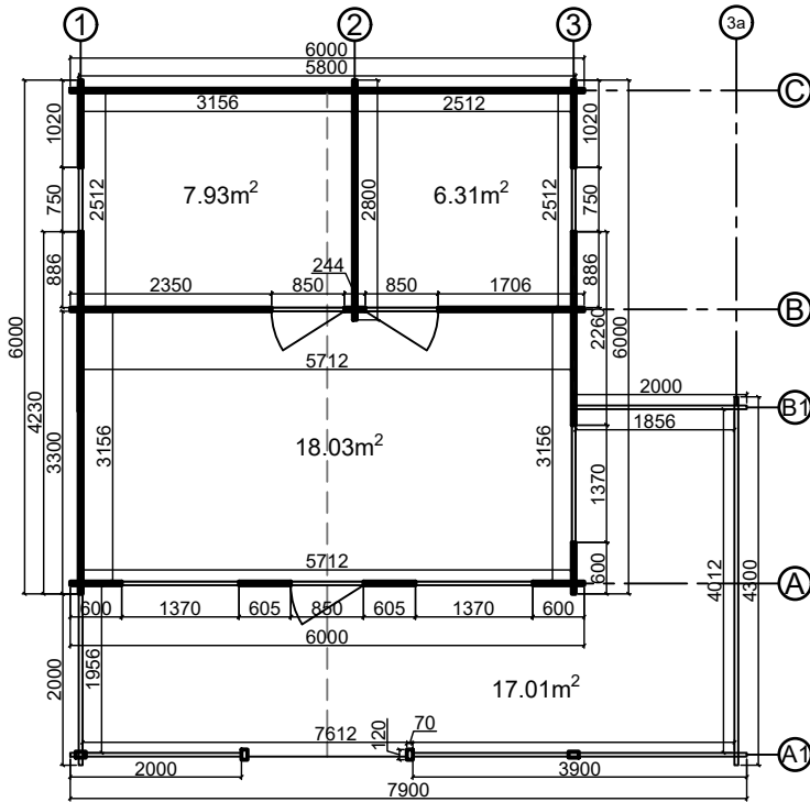
Floor plan
