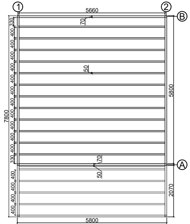
Base plan
