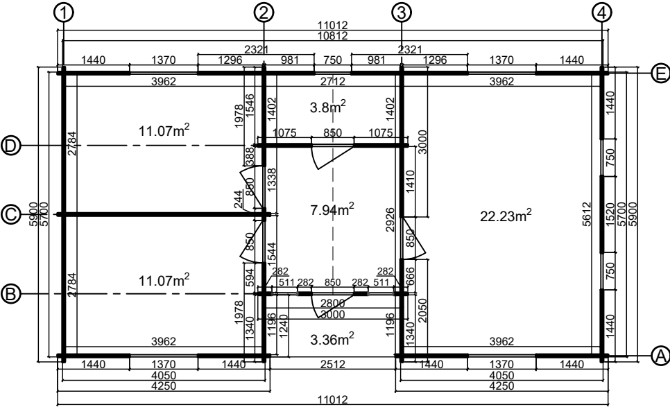
Floor plan
