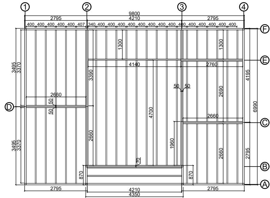
Base plan
