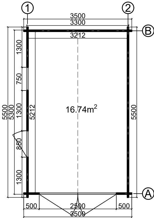
Floor plan
