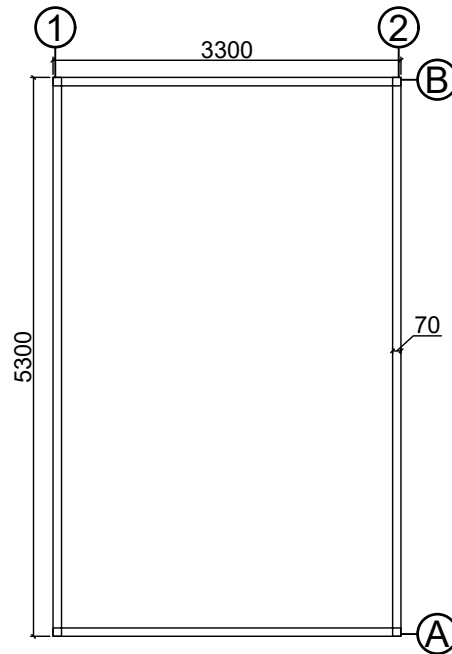
Base plan
